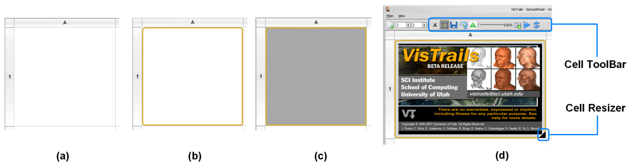
Figure 3.41: Different states of a spreadsheet cell. (a) inactive and unselected, (b) active and unselected, (c) active and selected, (d) an active cell with its toolbar and resizer.
