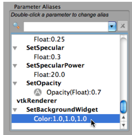
Figure 3.71: Creating the Background Alias.
