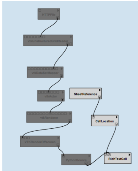
Figure 3.35: Pipeline - The results in the Pipeline view.
