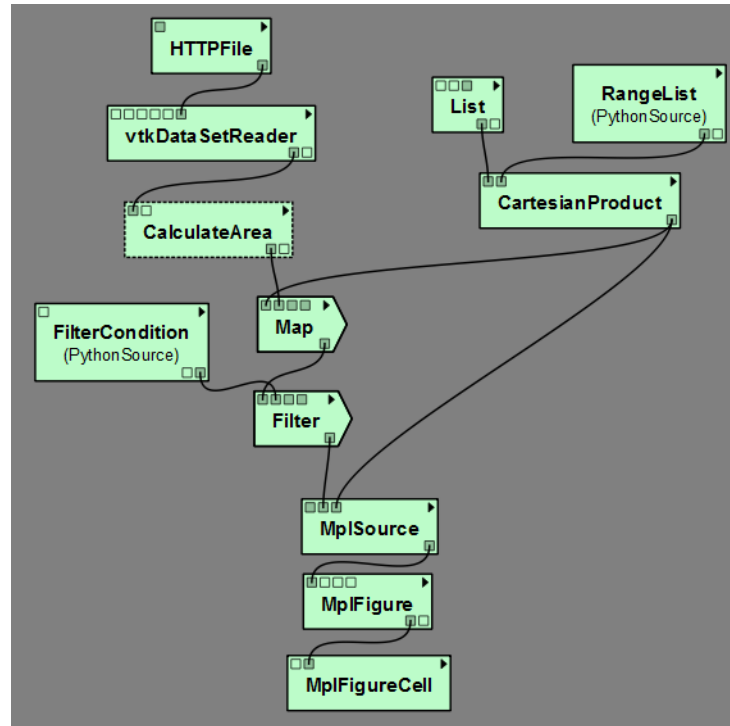
Figure 4.4: The new organization of the modules in the canvas
