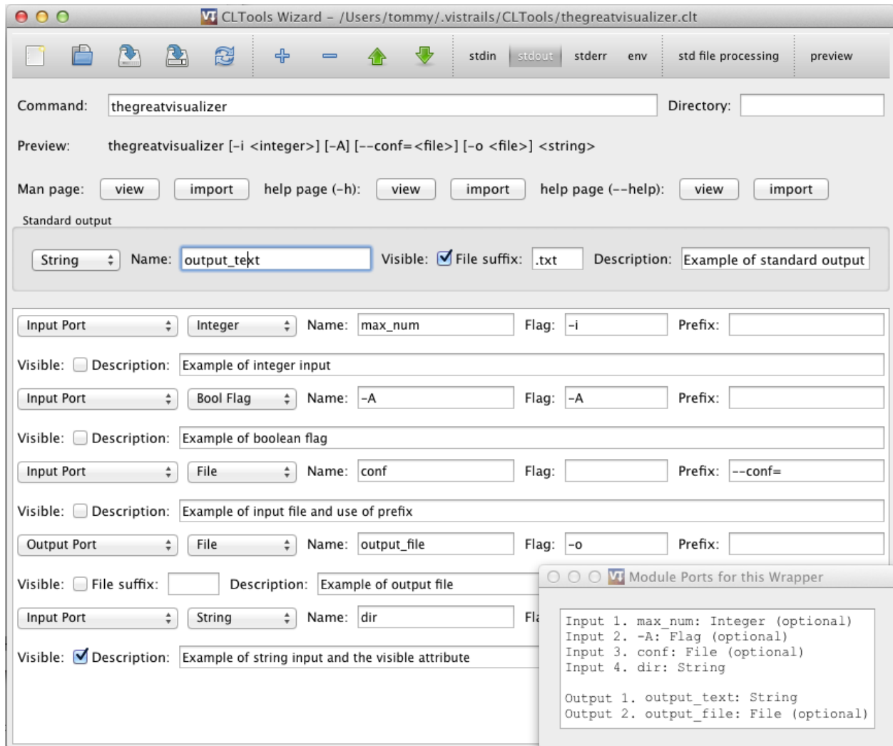
Figure 11.1: Figure 1.1 - CLTools Wizard main window
