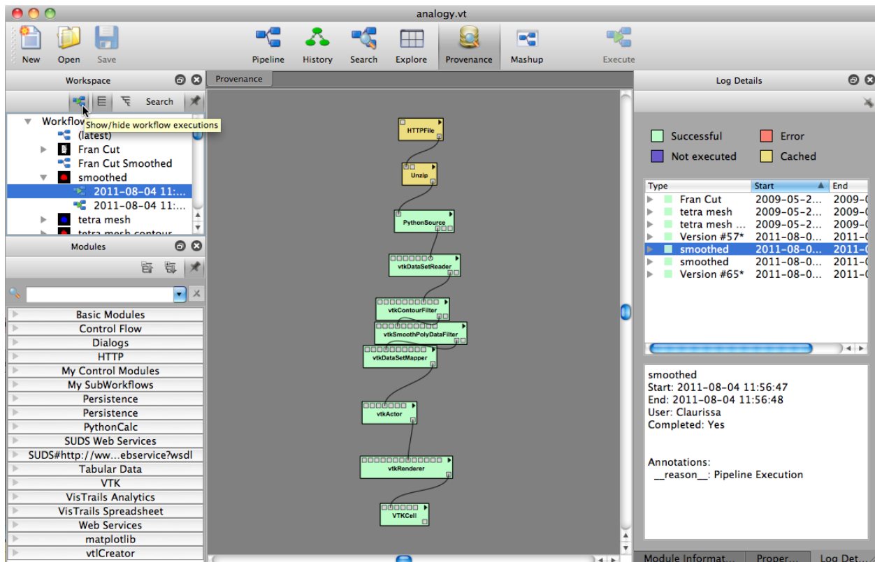
Figure 3.68: Provenance Browser - Left : The Workspace has a button to enable/disable executions. When enabled, executions of each tagged version in the vistrail will appear when each respective version is expanded. Right : The Provenance Browser keeps track of all executions whether they belong to tagged versions or not. When selected, the color coded execution pipeline will appear in the center panel.
