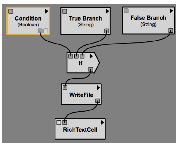
Figure 4.6: Simple If example
