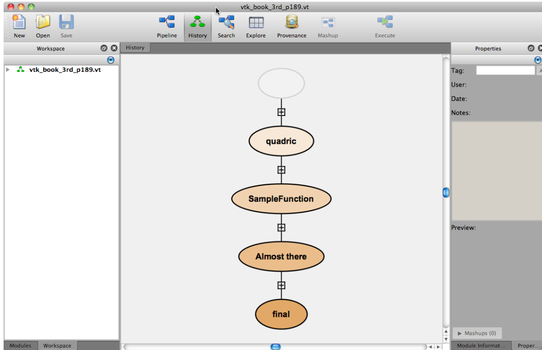
Figure 3.23: In History mode, you can examine and annotate different versions of a workflow.
