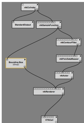
Figure 3.20: Renaming the group.
