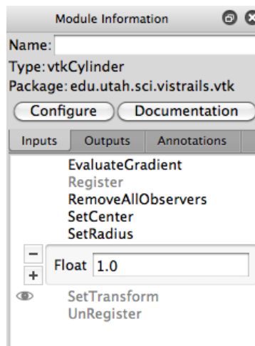
Figure 3.6: The module methods interface is shown with a change of the SetRadius parameter to 1.0.
