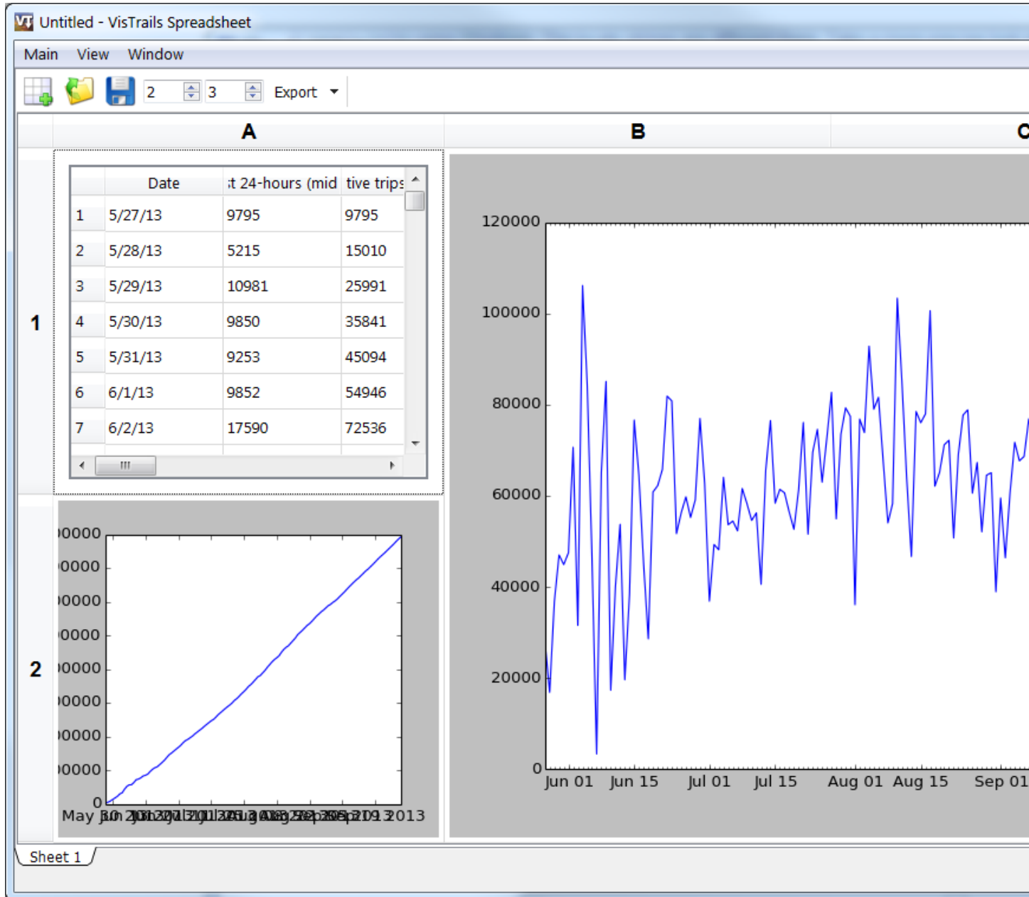
Figure 3.45: The result in the VisTrails Spreadsheet
