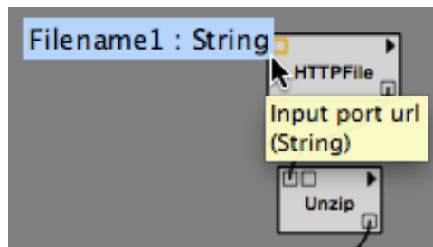
Figure 3.11: Assign a Variable - Drag the type from just below the Global Variables name on the Vistrail Variables tab. Drop it on a port to set the variable.
