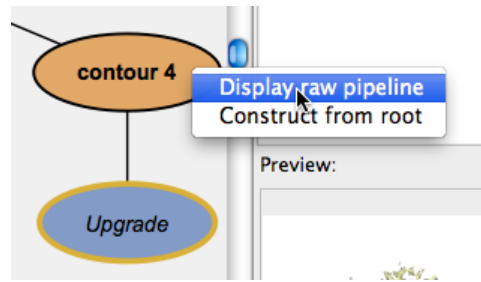
Figure 3.28: Original Pipeline - This figure shows how to view the original pipeline after an upgrade has occurred.
