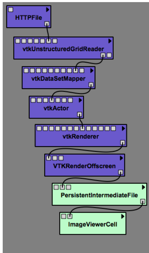
Figure 4.31: Example 1.5 - Persistent Intermediate File
