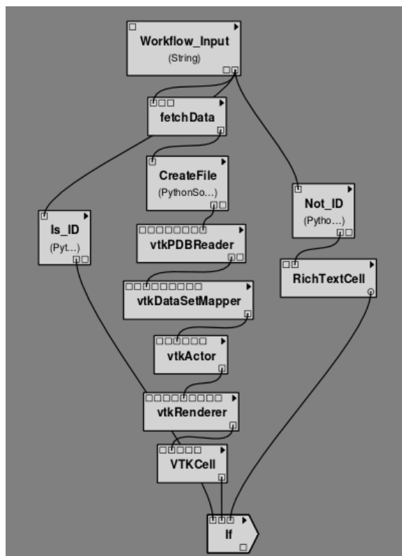
Figure 4.8: All the modules connected
