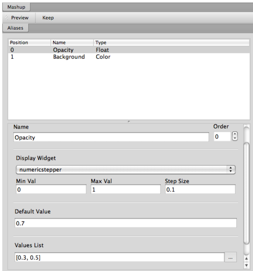
Figure 3.72: Configuring the Opacity alias.
