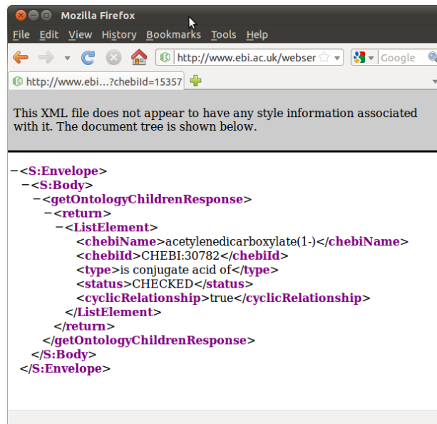
Figure 4.25: (b) Results from a “getOntologyChildren” query
