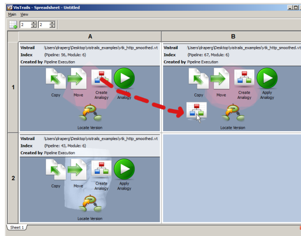
Figure 3.52: Drag the Create Analogy icon from the “source” cell to the “target” cell to create an analogy.
