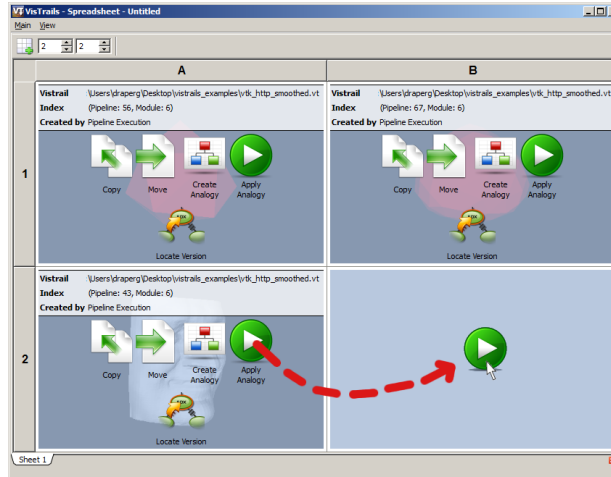
Figure 3.53: Drag the Apply Analogy icon from the cell you wish to modify to an empty cell.
