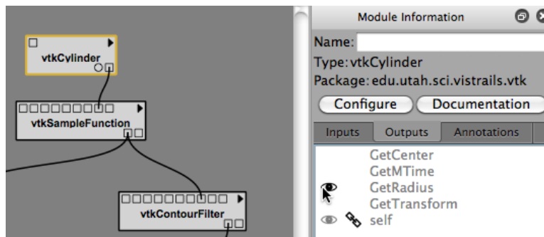
Figure 3.13: Enabling the GetRadius port from the Module Information tab.
