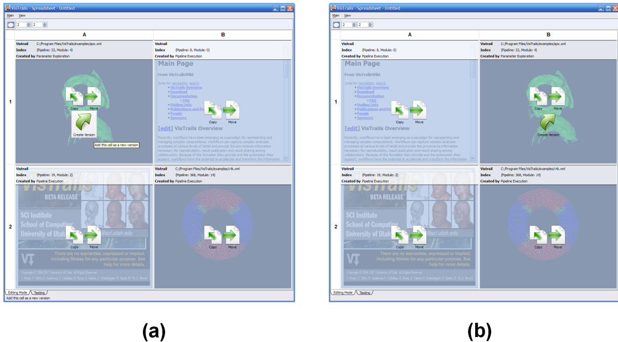
Figure 3.43: The spreadsheet in Editing Mode. (a) All cell widgets are replaced with an information widget (b) Two cells are swapped after drag and drop the ‘Move’ icon from A1 to B1.
