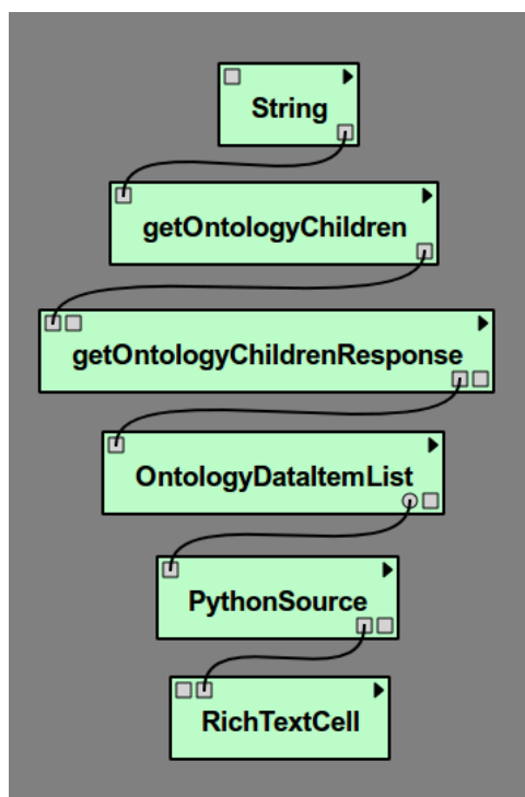
Figure 4.27: Our example pipeline
