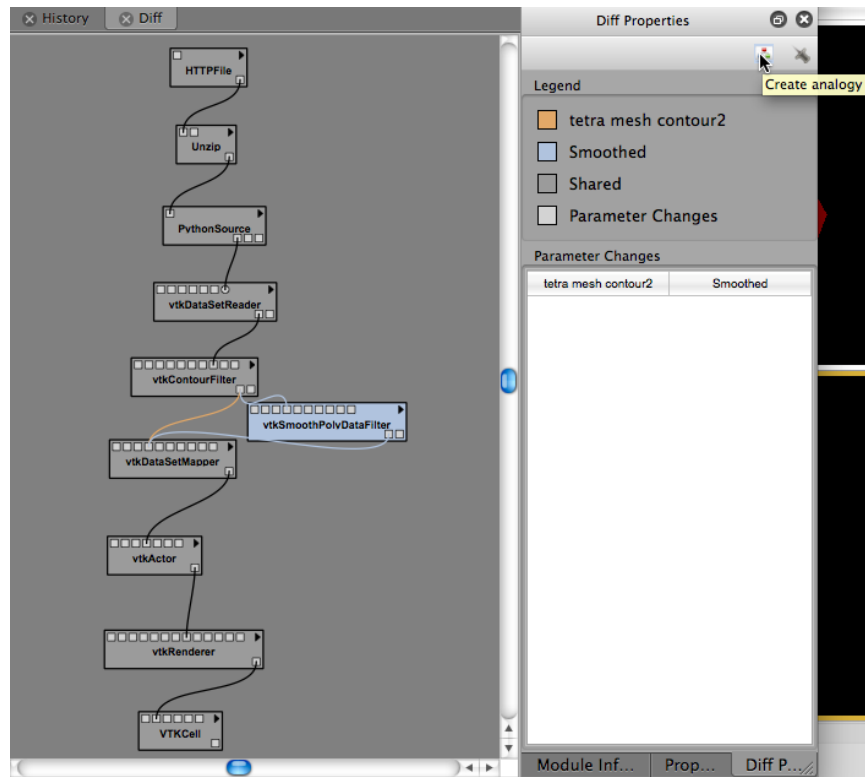
Figure 3.49: Click the Create Analogy button in the Diff Properties window to create a named analogy.
