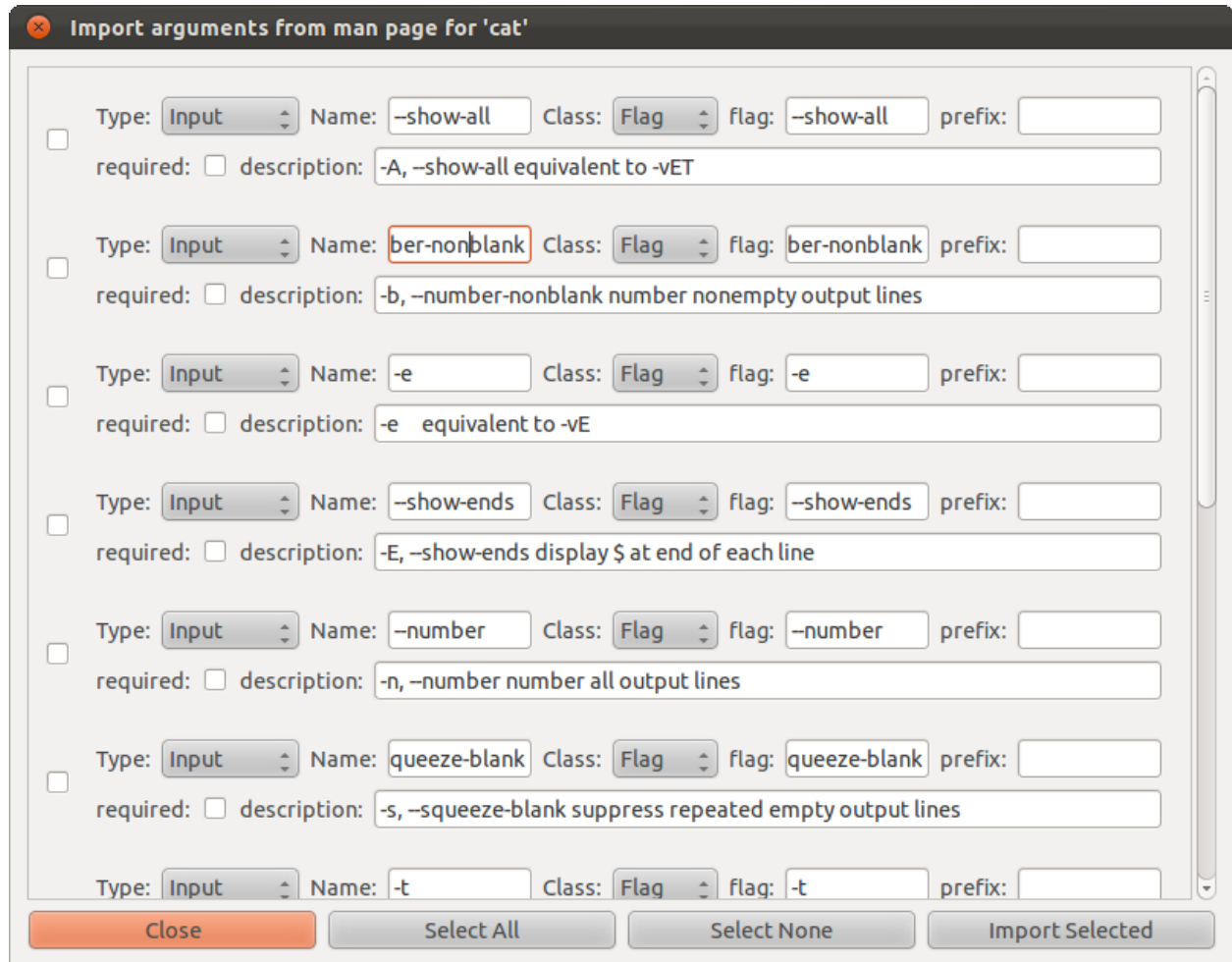
Figure 11.2: Figure 1.2 - Import Arguments Window
