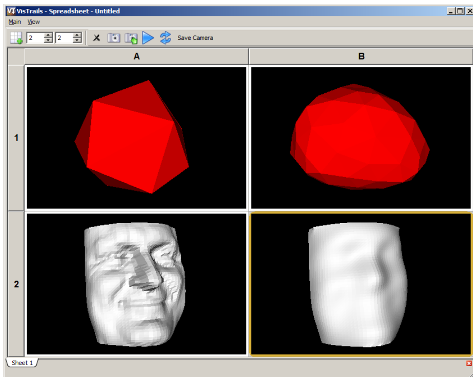
Figure 3.51: Result of applying a smoothing analogy to a different workflow.
