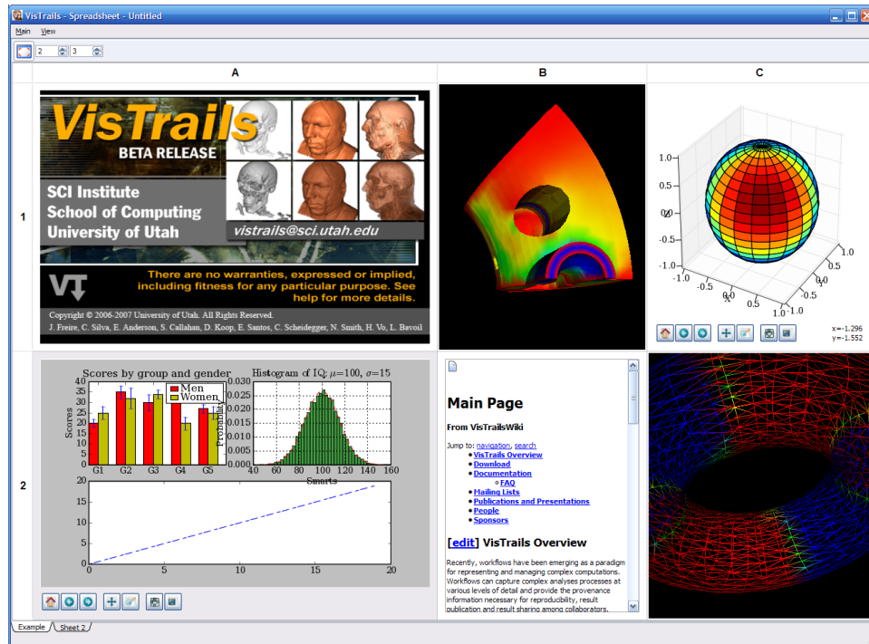
Figure 3.40: The VisTrails Spreadsheet.
