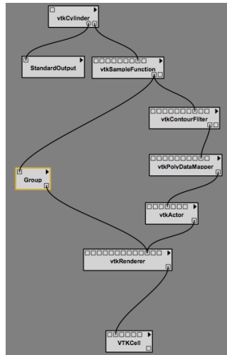
Figure 3.19: The modules represented as a single group module.
