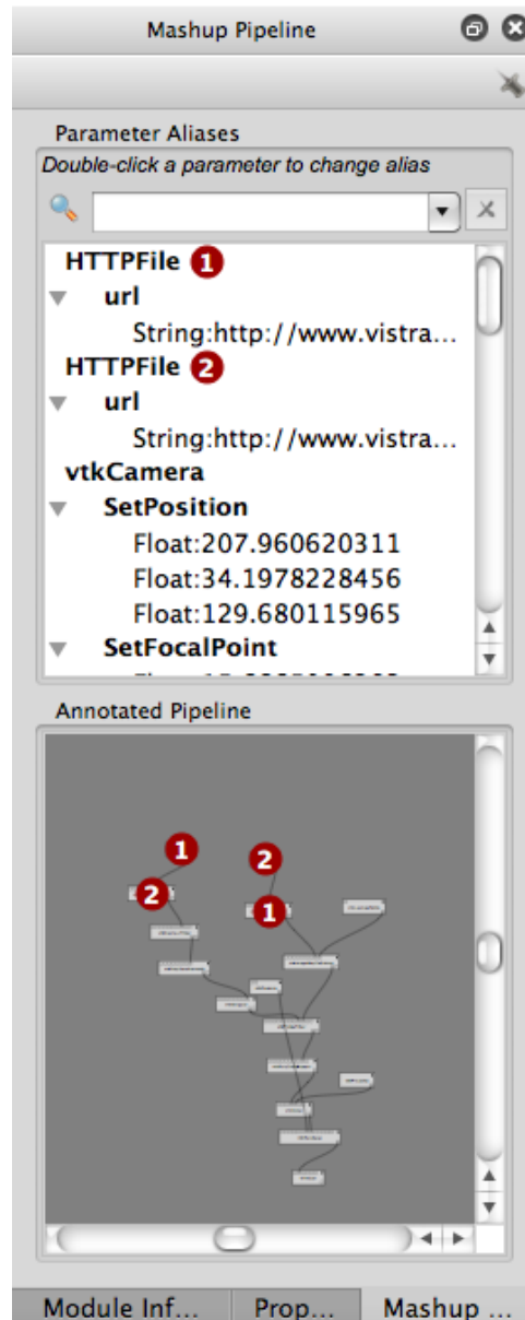
Figure 3.69: Numbered Modules - The HTTPFile modules 1 and 2 appear in the annotated pipeline and in the parameter aliases. The annotated pipeline also, numbers the vtkDataSetReader modules (which appear below the respective HTTPFile modules in the pipeline). Their parameters have not been exposed to the mashup, so they do not appear in the Parameter Aliases section.
