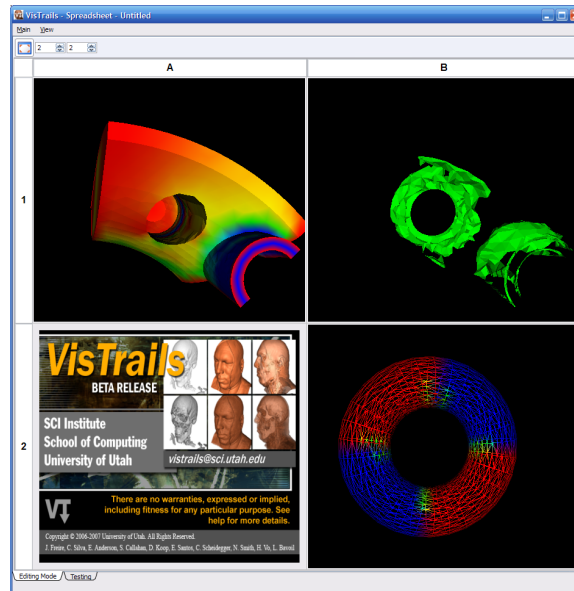
Figure 3.42: When selecting all cells, interacting with one VTK cell (A1) causes the other two VTK cells (B1 and B2) to change their camera to the same position.
