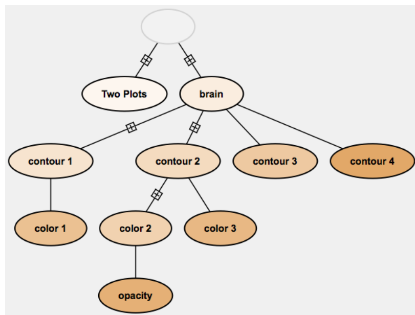
Figure 3.31: The resultant history tree.
