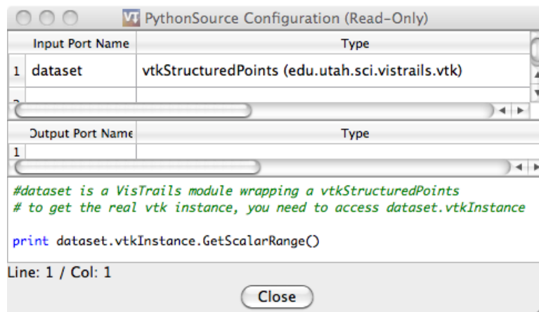
Figure 3.17: Accessing vtkObjects - The vtkObject of a VTK module, ‘dataset’, is accessed with ‘dataset.vtkInstance’.
