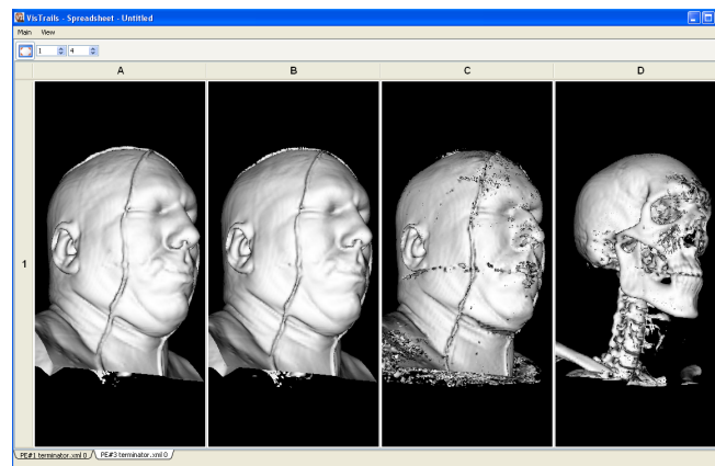
Figure 3.56: Parameter Exploration of four isovalues as displayed in the Spreadsheet.
