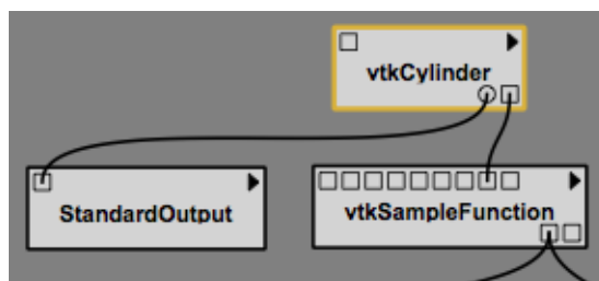
Figure 3.14: The vtkCylinder module is configured to show an additional GetRadius port, which is then connected to a StandardOutput module.
