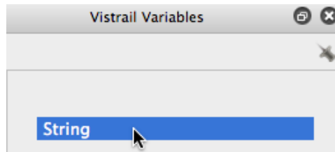
Figure 3.10: Create a Variable - Drag the String module and drop it in the Vistrail Variables tab to create a global variable.
