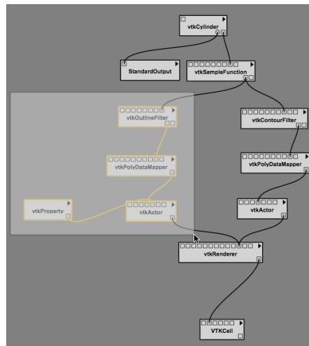
Figure 3.18: Box selection of four modules.
