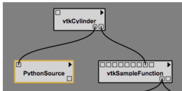
Figure 3.15: A PythonSource module can be used to directly insert scripts into the workflow.
