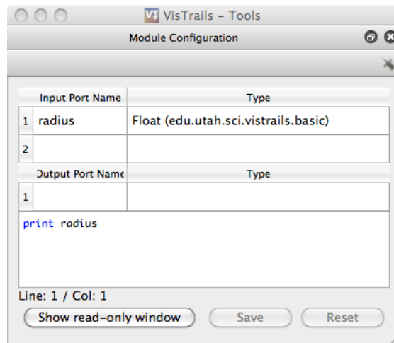
Figure 3.16: The configuration window for PythonSource allows multiple input and output ports to be specified along with the Python code that is to be executed.
