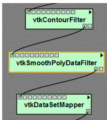
Figure 3.46: Modified pipeline for use in our example.
