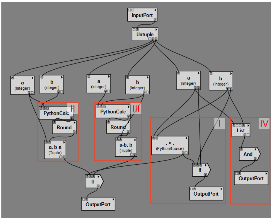
Figure 4.12: The grouped pipeline for Euclid's algorithm
