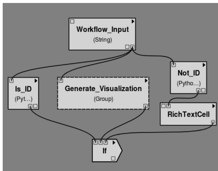
Figure 4.9: The final workflow, using the Group structure
