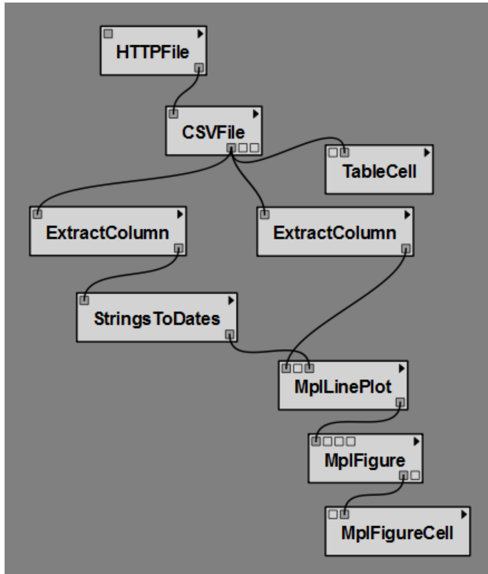
Figure 3.44: The pipeline for the Bikes example
