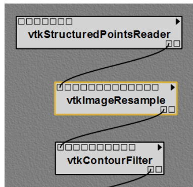
Figure 3.57: Inserting a vtkImageResample module into the "terminator.vt" example pipeline.
